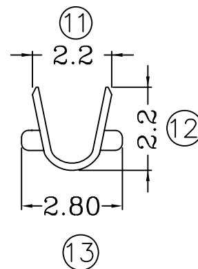
Section C-C
